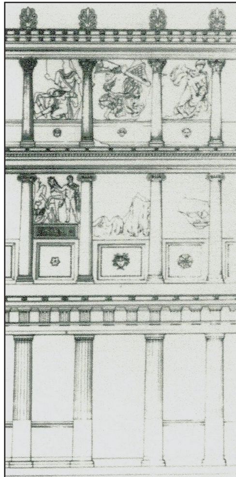
Figure 1: Partial reconstructed elevation of South Portico
